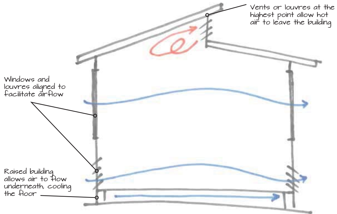
Figure 1. Passive Ventilation (cross-section)
