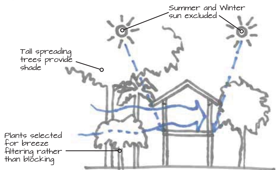
Figure 5B. Shading and Landscaping
