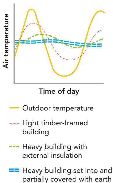
Figure 6. Diurnal temperature range and response of low and high thermal mass materials
