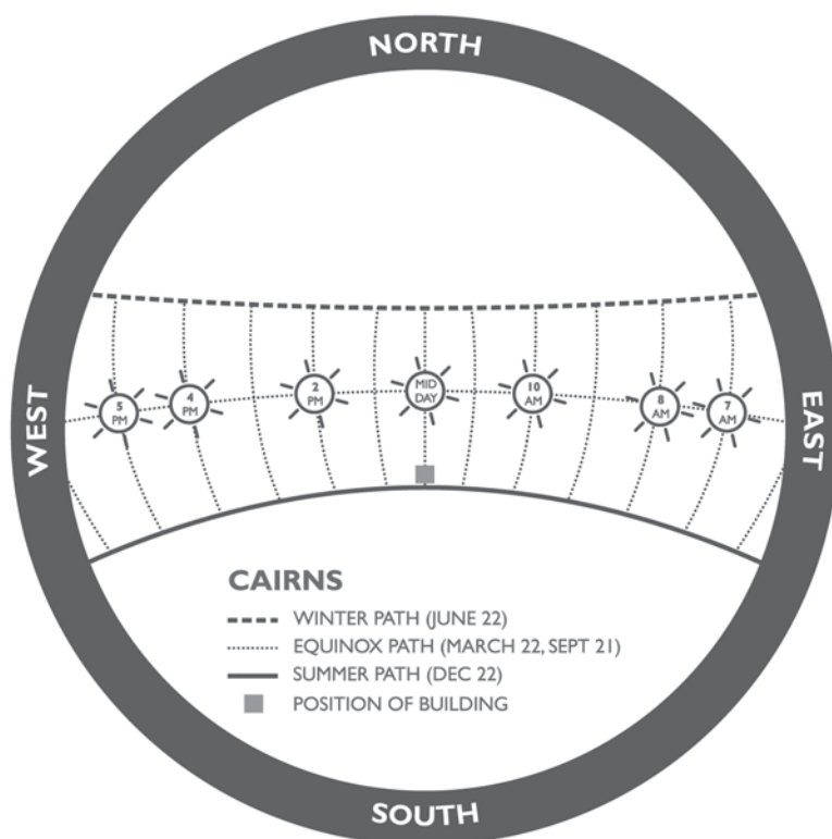
Figure 2. Sun path diagram for the Cairns Region
