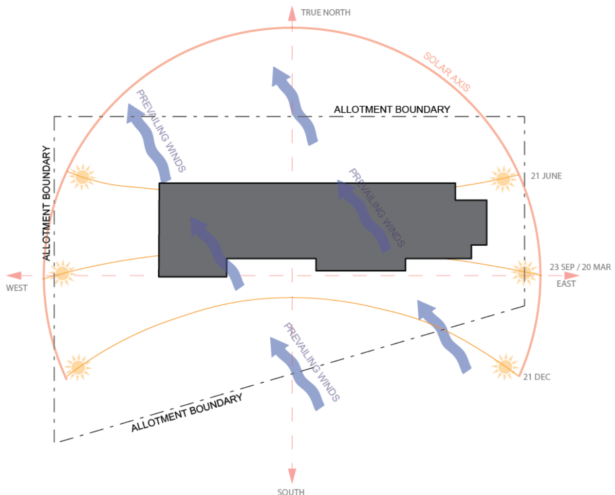
Figure 11 Site analysis overlaid with the building footprint
