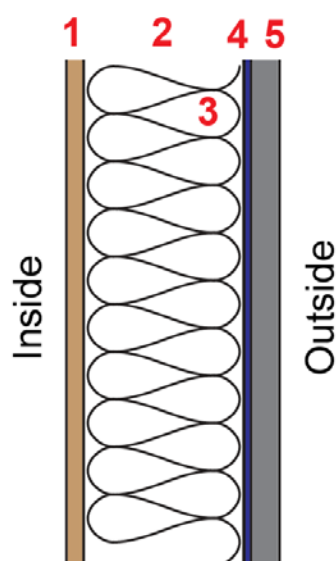
Figure 5 Typical external wall cross section
