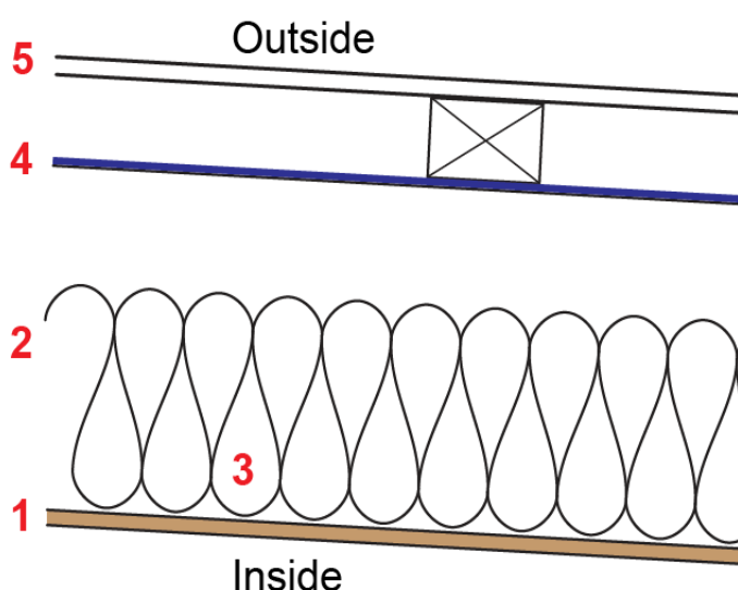
Figure 4 Typical roof section
