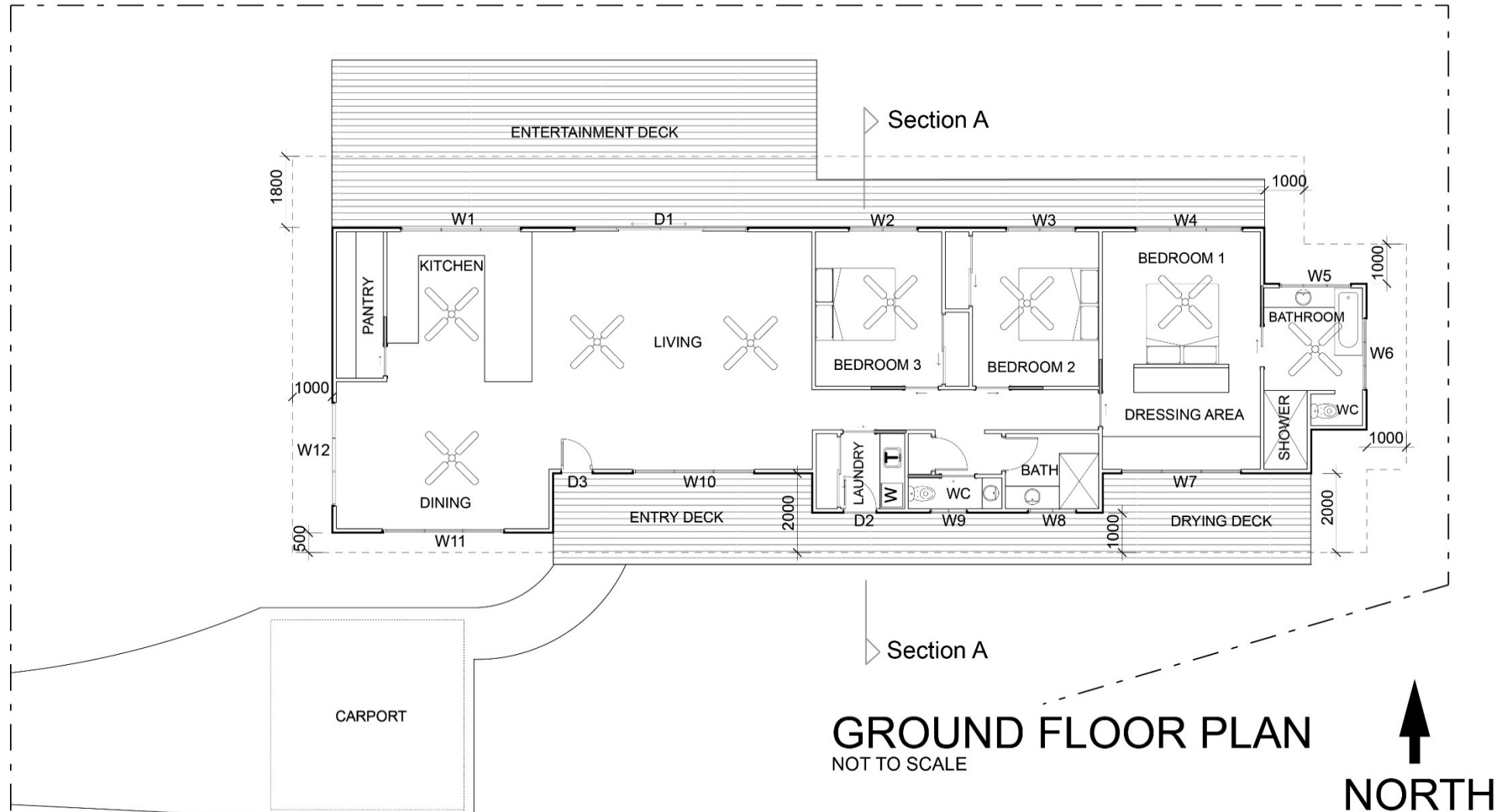
Figure 1 Plan view of the design
