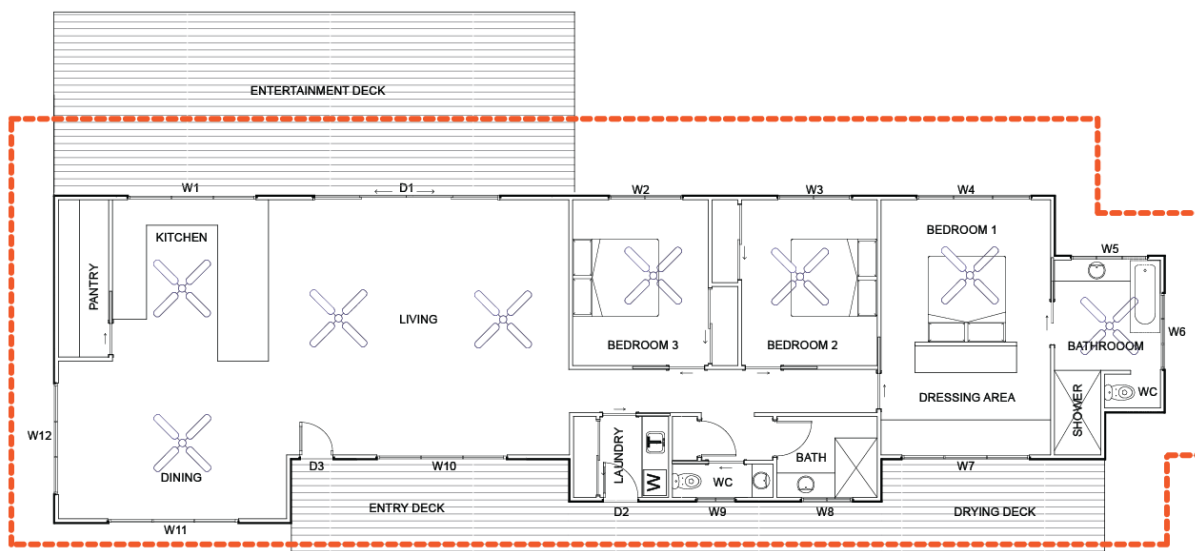
Figure 10 Orange dotted line shows the external footprint of the roofs eave lines around the building.
