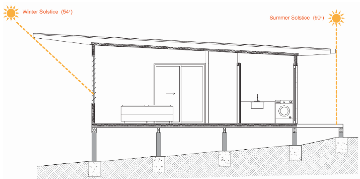
Figure 9 Winter and summer solstice sun angles
