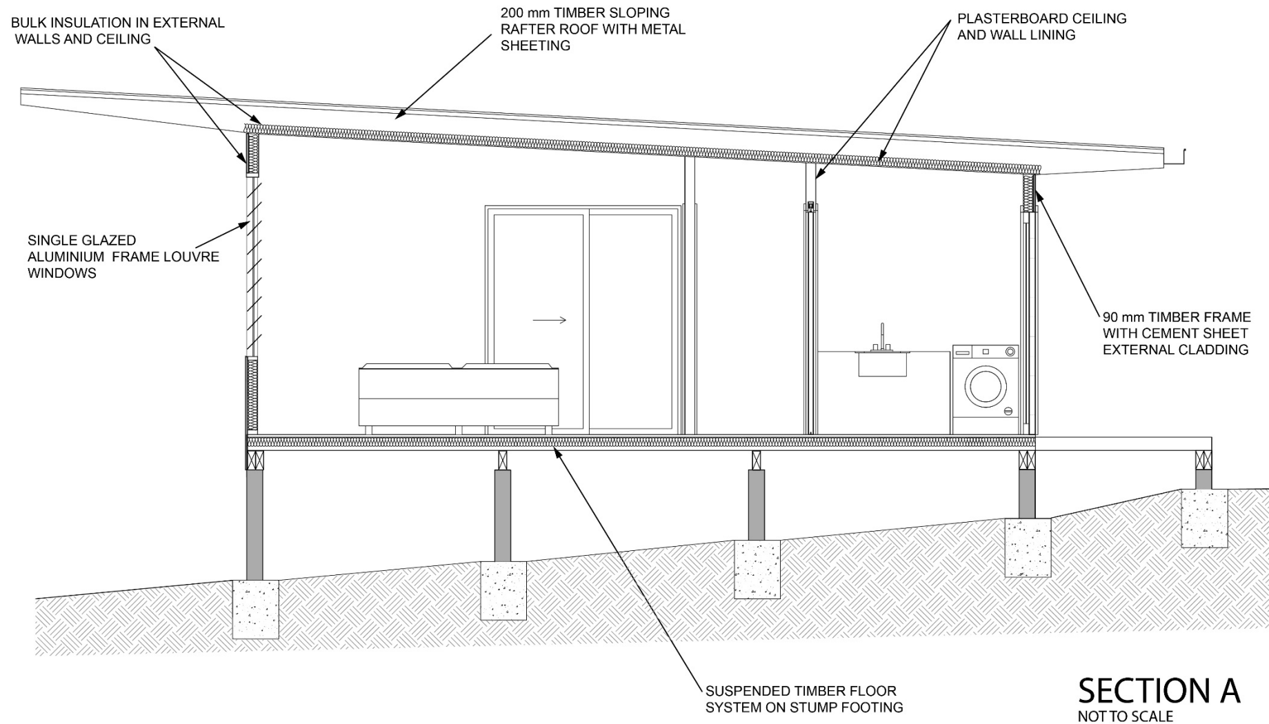
Figure 2 Section view of the design
