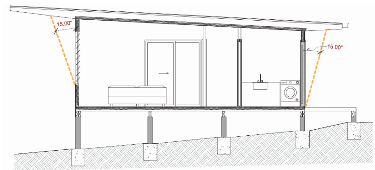
Figure 6 Shading of external walls
