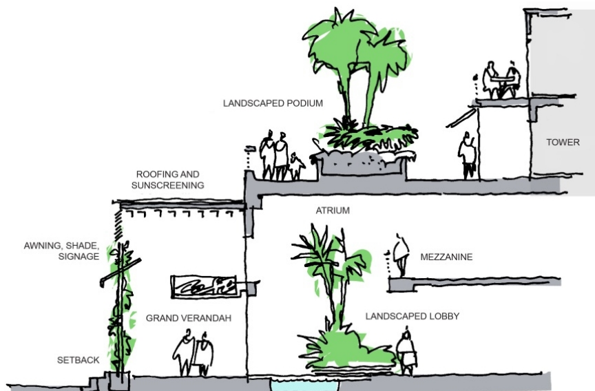
Figure SC6.16.3.8.d – Street canopy (typical cross section)
